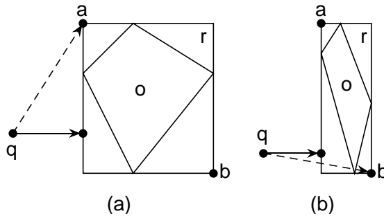
Fig. 8. An example of \text{MINDIST} (solid line) and \text{MINMAXDIST} (broken line) for a bounding rectangle r . The distance of the object o from q is bounded from below by \text{MINDIST}(q, r) and from above by \text{MINMAXDIST}(q, r) . Notice that in (b) point b is closer to q than point a , while this is not the case in (a).
