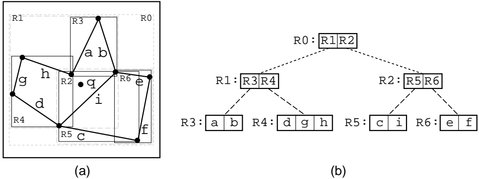
Fig. 1. An R-tree index for a set of nine line segments. (a) Spatial rendering of the line segments and bounding rectangles; (b) a tree access structure for (a). In the interest of clarity, the bounding rectangles for the individual line segments are omitted from (a).
