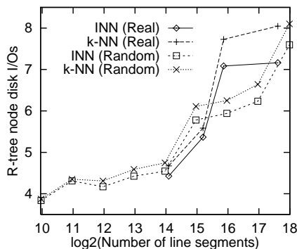
Fig. 25. R-tree node disk I/Os for finding one neighbor.
