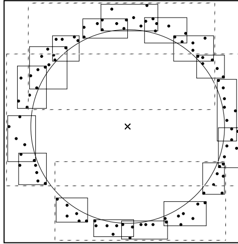
Fig. 6. An example of an R-tree of points with node capacity of 8, showing a worst case for nearest neighbor search.
