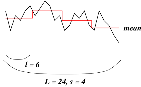
Figure 2: Example of Segmented Means
