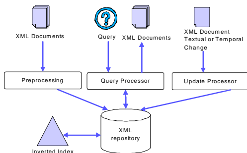
Fig. 3. The overall system architecture
