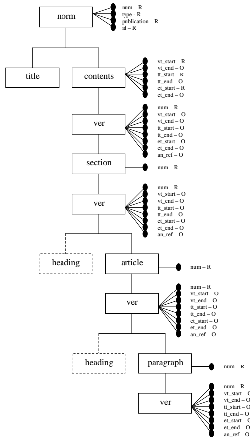
Fig. 1. The XML-schema for the representation of norms in time
